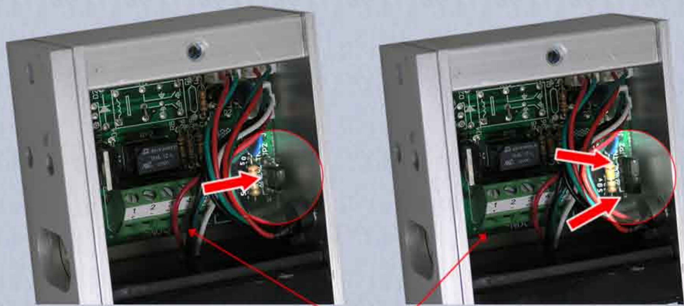
Jumper Setting for 24VDC Operation
